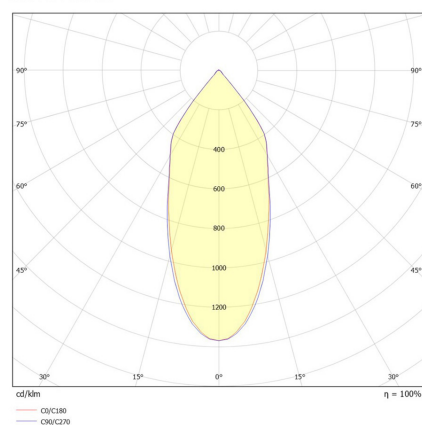
Monza Duo 50°
