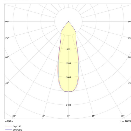
Monza Duo 40°
