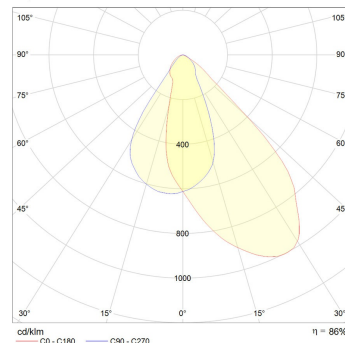
Capella Wall Washer 55°
