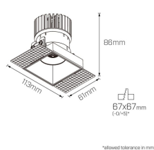
Bron Square Fixed Trimless 7W
