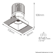
Bron Square Fixed Trimless 7W
