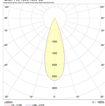
*Bron 7W/13W/18W 30°
