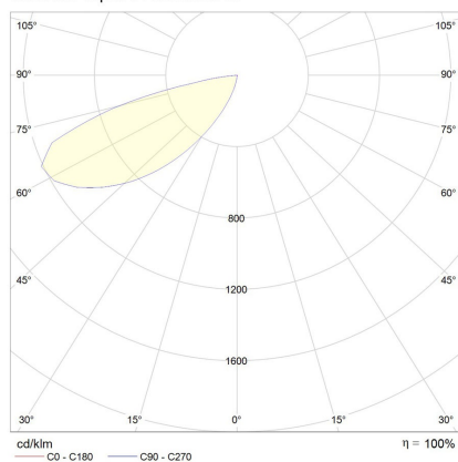
Toulouse Square Recessed 45°
